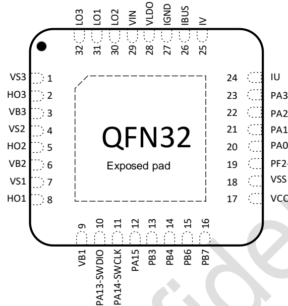
图 3-1 QFN32(4*4) Pinout1 PY32MD420K1xU (Top View)
