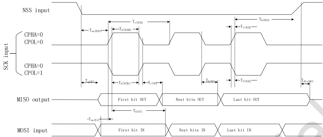
图 5-1 SPI 时序图—Slave mode and CPHA=0
